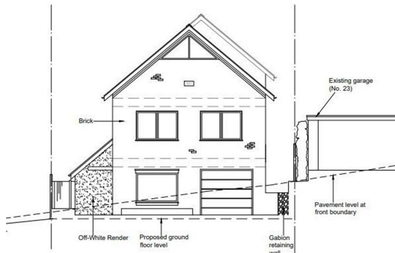
Front Elevation (North West)
